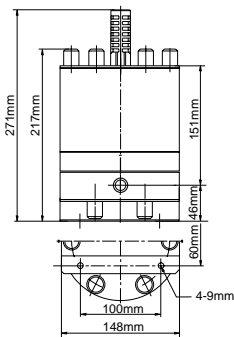
AD-25TT
