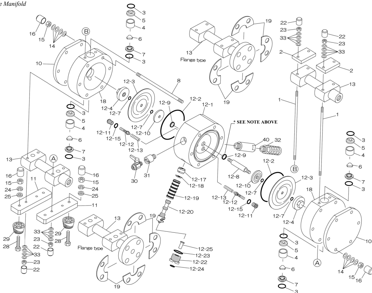
Flange Manifold
