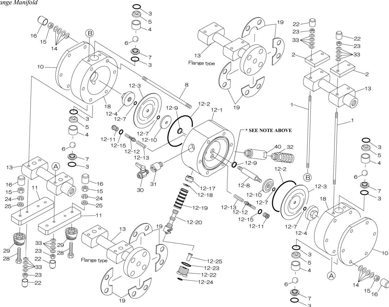
Flange Manifold
